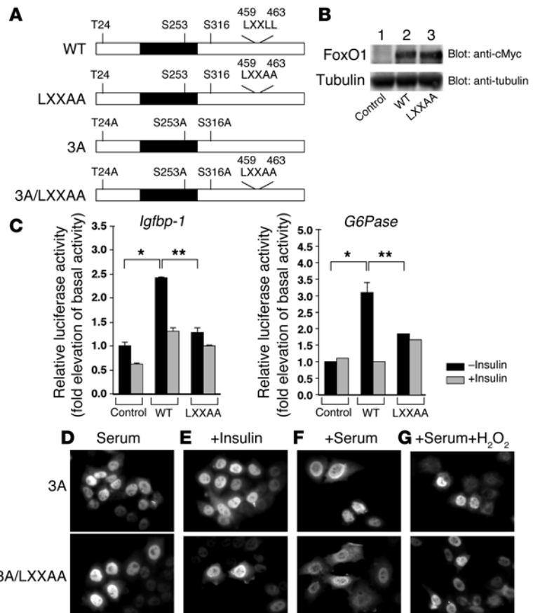
Figure 1 Scheme and subcellular localization of FoxO1 mutants in SV40-transformed hepatocytes and expression of an Igfbp-1 /luciferase or G6Pase /luciferase reporter gene in SV40-transformed hepatocytes transfected with WT or LXXAA FoxO1. (A) Scheme of WT, LXXAA FoxO1, 3A FoxO1, and 3A/LXXAA FoxO1. (B) Expression of cMyc-WT (lane 2) and LXXAA FoxO1 (lane 3) in SV40-transformed hepatocytes was detected. (C) After overnight serum deprivation and induction with dexamethasone, 8-Br-cAMP, and IBMX in the presence or absence of insulin (100 nM) as described in Methods, cells were harvested and luciferase activity was measured. *Statistically significant difference between control and WT-transfected cells, P < 0.001 by 1-way ANOVA; **statistically significant difference between WT- and LXXAA-transfected cells, P < 0.005 by 1-way ANOVA. Data represent mean \pm SEM from 3 independent transfection experiments. Following transient transfection, hepatocytes were seeded onto 4-well slide culture chambers and incubated in various conditions, including serum deprivation, for 24 hours (D), stimulation with insulin (100 nM, 20 minutes) (E), incubation with serum (F), and stimulation with H 2 O 2 (250 \mu M, 4 hours) (G). Myc epitope-tagged FoxO1 was visualized with anti-cMyc monoclonal antibody and FITC-conjugated anti-mouse IgG.
