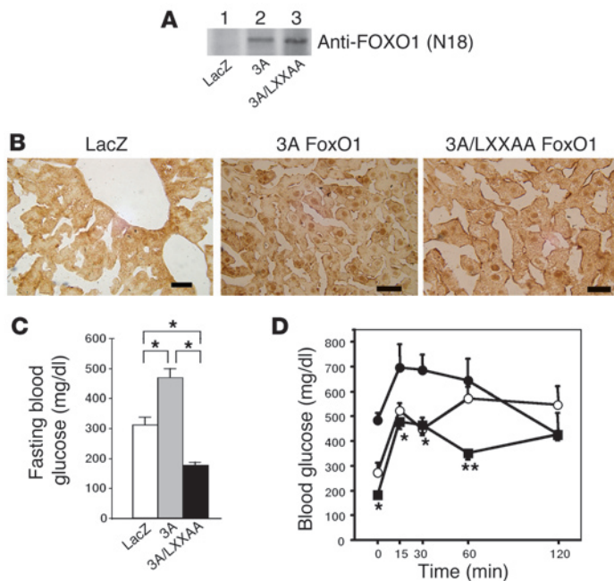
Figure 9 Effects of overexpression of 3A/LXXAA FoxO1 on fasted blood glucose and glucose tolerance in Lep r db/db mice. (A) Expression of 3A FoxO1 or 3A/LXXAA FoxO1 mutant in liver. Liver was removed from mice at day 5 after injection with adenovirus encoding LacZ (lane 1), 3A FoxO1 (lane 2), or 3A/LXXAA FoxO1 (lane 3) intravenously, and 15 \mu g of each liver lysate was subjected to immunoblot analysis with an anti-FOXO1 polyclonal antibody (N18). (B) Immunohistochemistry of liver from Lep r db/db mice injected with adenovirus encoding LacZ (left panel), 3A FoxO1 (middle panel), or 3A/LXXAA FoxO1 (right panel). Each panel shows representative sections. Magnification, \times 40 . Scale bar: 10 \mu m. (C) Effect of overexpression of 3A FoxO1 or 3A/LXXAA FoxO1 in liver from Lep r db/db mice on fasted blood glucose. Blood glucose levels were measured as described in Methods after overnight fasting at day 5 after injection with each adenovirus encoding LacZ (white bar), 3A FoxO1 (gray bar) or 3A/LXXAA FoxO1 (black bar). Data represent mean \pm SEM of 6 mice for each group. *Statistically significant difference between mice injected with each adenovirus encoding LacZ, 3A FoxO1, or 3A/LXXAA FoxO1. P < 0.001 by 1-way ANOVA. (D) Intraperitoneal glucose tolerance test was performed in mice injected with the adenoviruses indicated. The groups of mice indicated were injected with a 1.2 g/kg of body weight of glucose intraperitoneally as follows: LacZ (open circles, n = 6 ), 3A FoxO1 (filled circles, n = 6 ), and 3A/LXXAA FoxO1 (filled squares, n = 6 ). *Statistically significant difference between 3A and 3A/LXXAA, P < 0.01 by 1-way ANOVA; **statistically significant difference between 3A/LXXAA and LacZ or 3A, P < 0.01 by 1-way ANOVA.
