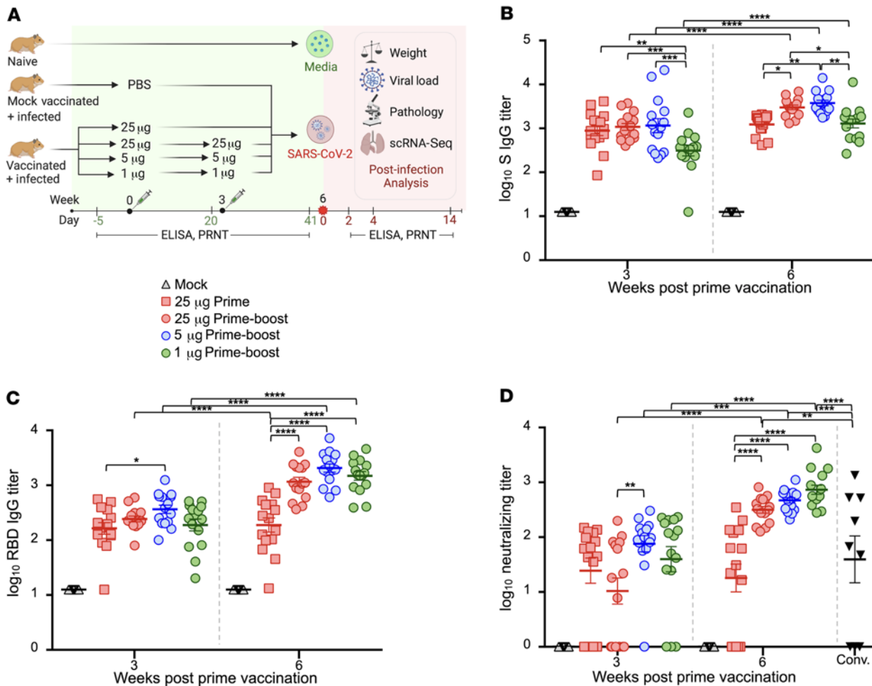
Figure 1. Serum antibody responses in vaccinated hamsters. (A) Study design. Hamsters were prime-vaccinated via the i.m. route at week 0 and boosted at week 3, with 25 μg ( n = 15 ), 5 μg ( n = 15 ), and 1 μg ( n = 15 ) of mRNA-1273. A group of hamsters ( n = 15 ) received a prime dose only of 25 μg mRNA-1273, and a mock group received PBS ( n = 15 ) at week 0. At week 6, animals were intranasally challenged with 10^5 PFU of SARS-CoV-2. On days 2, 4, and 14 after infection, hamsters ( n = 5 per group) were euthanized for tissue collection. PRNT, plaque reduction neutralization test (B–D) Total serum SARS-CoV-2 S-specific (B) and RBD-specific (C) IgG titers in serum and neutralizing titers (D) in hamster groups prior to SARS-CoV-2 infection measured by ELISA and plaque reduction assays, respectively. Neutralizing titers were compared with a panel of human convalescent serum samples (Conv.). Bars denote group means \pm SE. Significance was measured by ANOVA with Tukey’s or Šidák’s correction for multiple comparisons between vaccine groups or between time points, respectively ( *P \leq 0.05 , **P \leq 0.01 , ***P \leq 0.001 , ****P \leq 0.0001 ).
